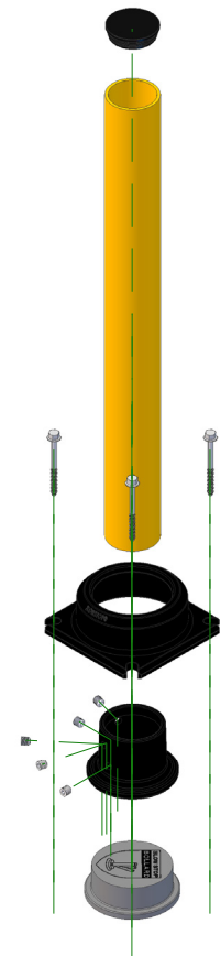
Exploded
