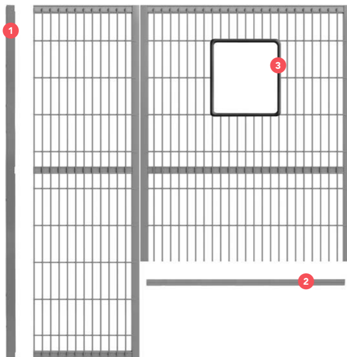
PC HOLDER The PC holder fix a polycarbonate infill sheet to the mesh panel, to withhold liquids and small parts.
