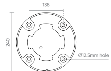
Receiver Plate
