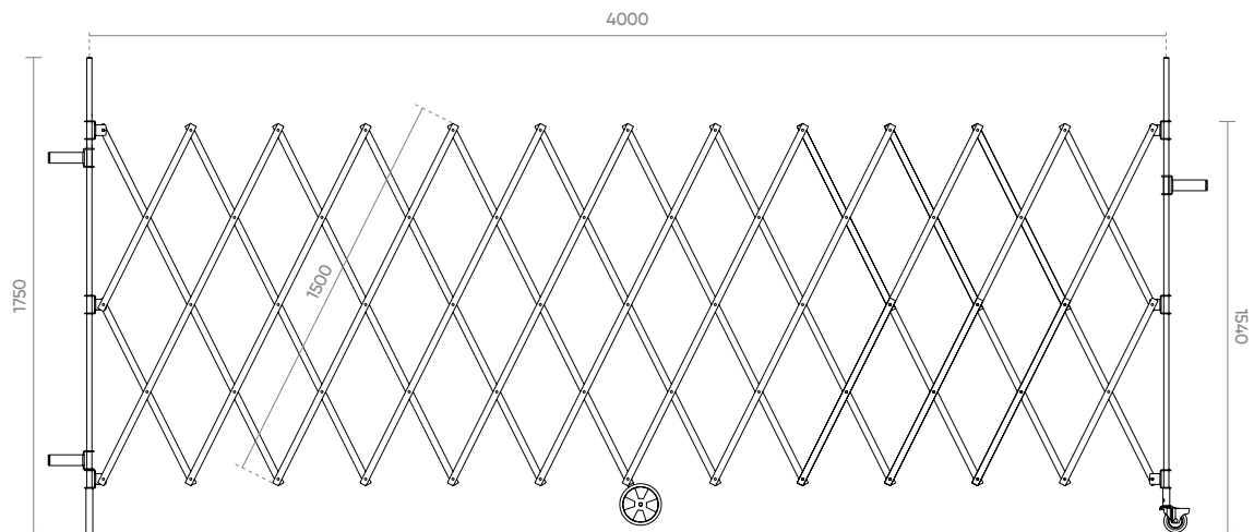
SpanSafe Wall Mount Expandable Barrier, 1500mm x 4m wide (2714-146)
