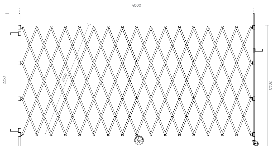
SpanSafe Wall Mount Expandable Barrier, 2000mm x 4m wide (2714-170)
