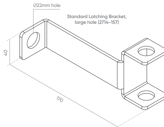
Latch to Join Two Barriers Together (optional extra)
