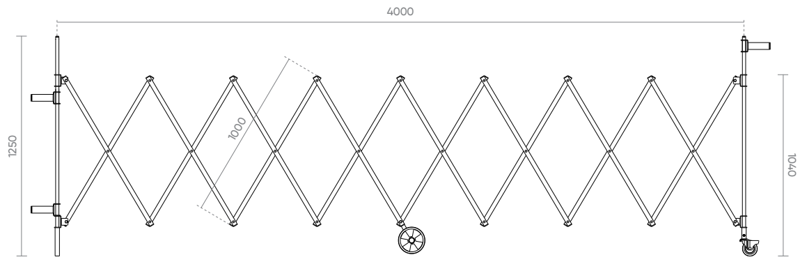
SpanSafe Wall Mount Expandable Barrier, 1000mm x 4m wide (2714-144)
