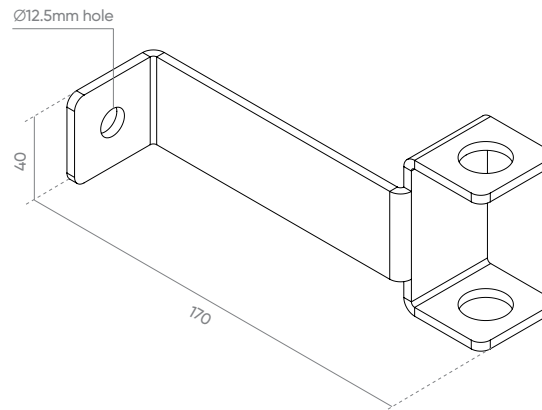
Wall Bracket, small hole (2714-156) 2 supplied with every barrier
