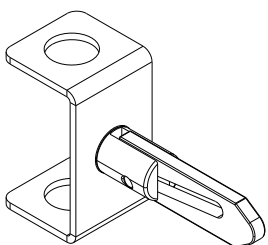
Gate Mounted Drop Latch (2714-165)
