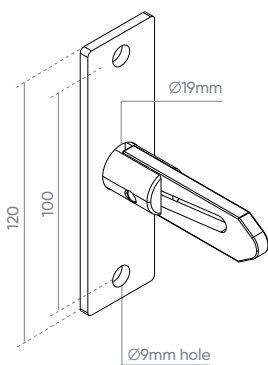
Wall Mounted Drop Latch (2714-158)
